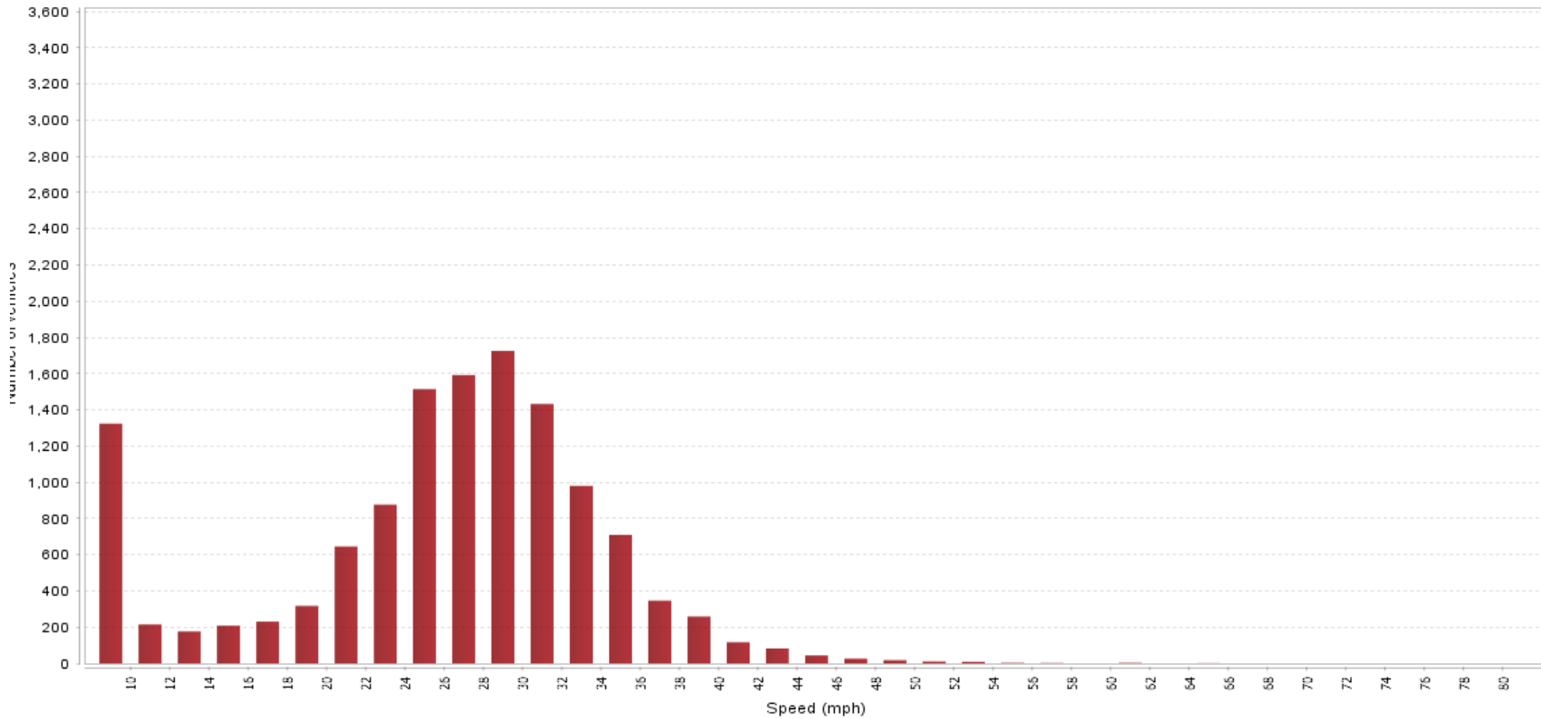
Velocity Histogram -- Period of analysis : Sun 1. Oct 2023, 00:00 o'clock -till- Tue 31. Oct 2023, 23:59 o'clock
